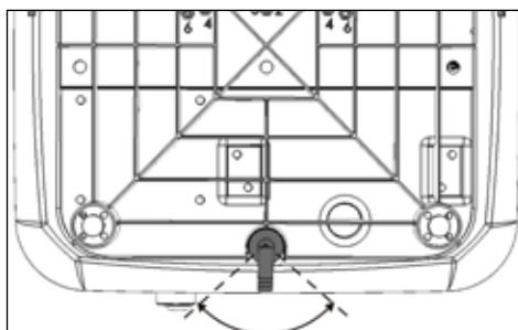
Condensate drainage orientation (seen from below the appliance)
